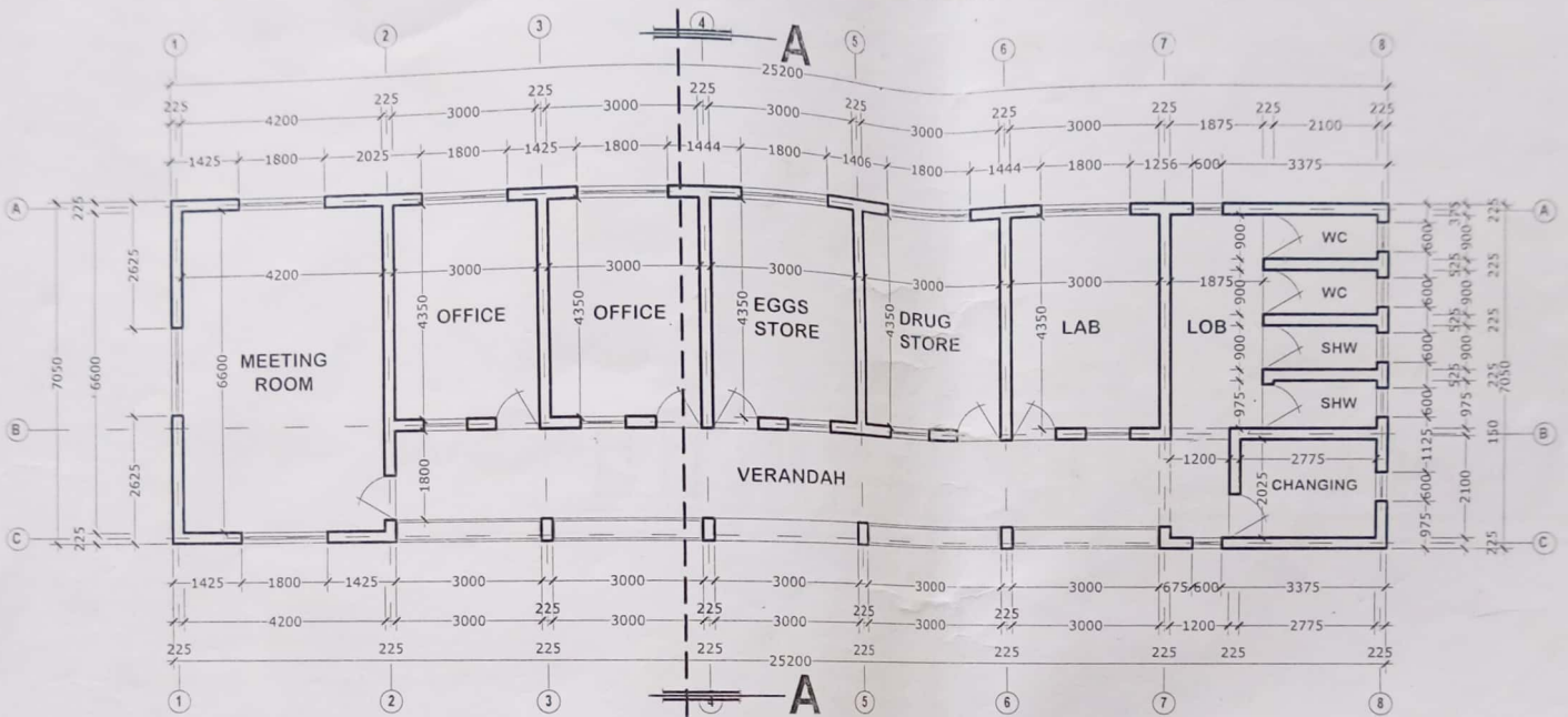
ADMIN OFFICE(floor plan)
