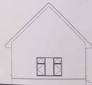
LEFT ELEVATION
