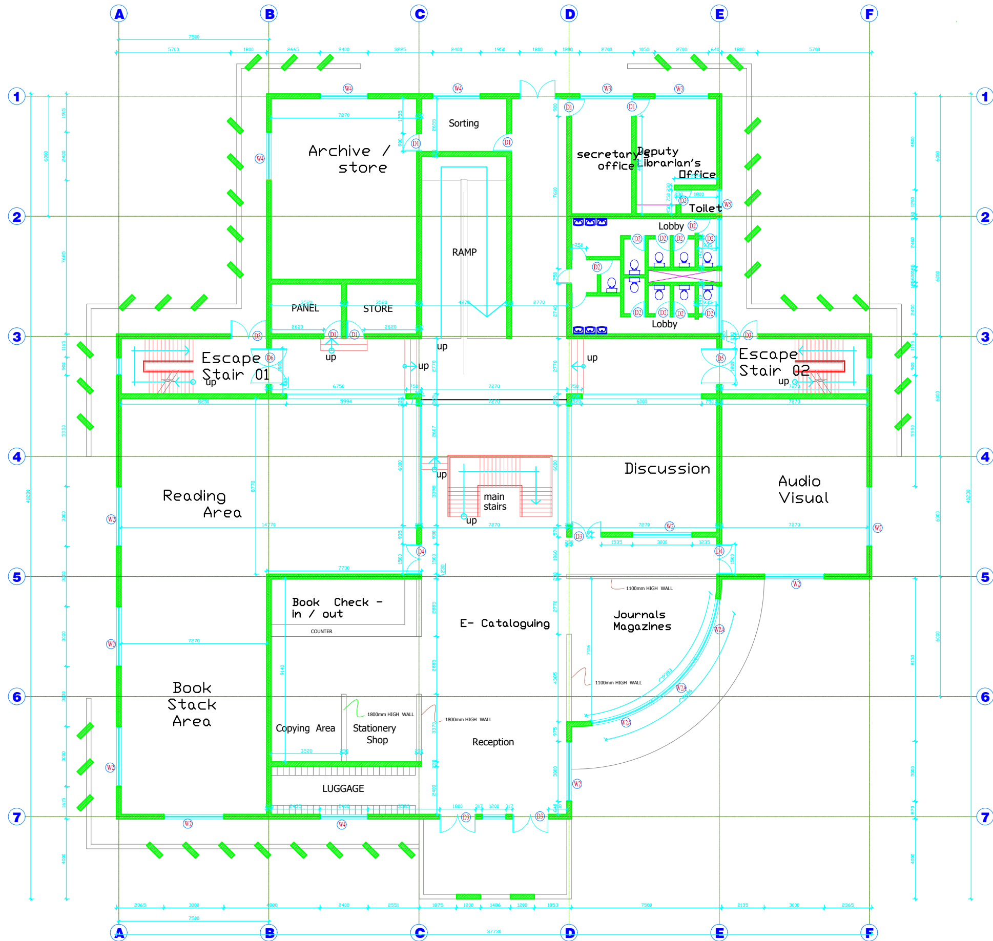
GROUND FLOOR PLAN (School Library)
