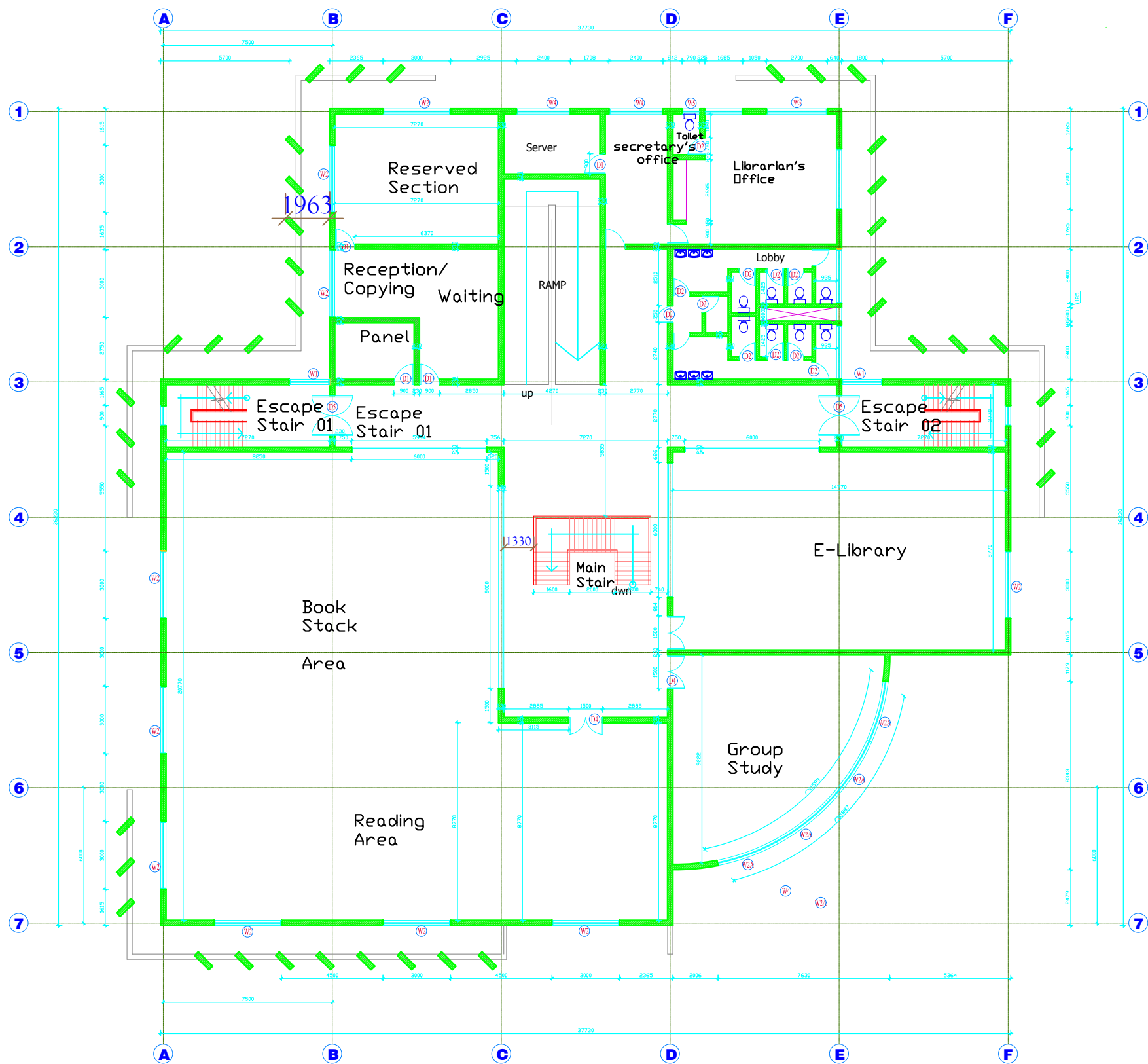
FIRST FLOOR PLAN (School Library)
