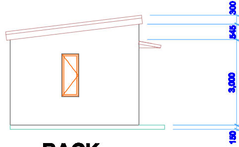
BACK ELEVATION
