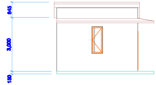
LEFT ELEVATION
