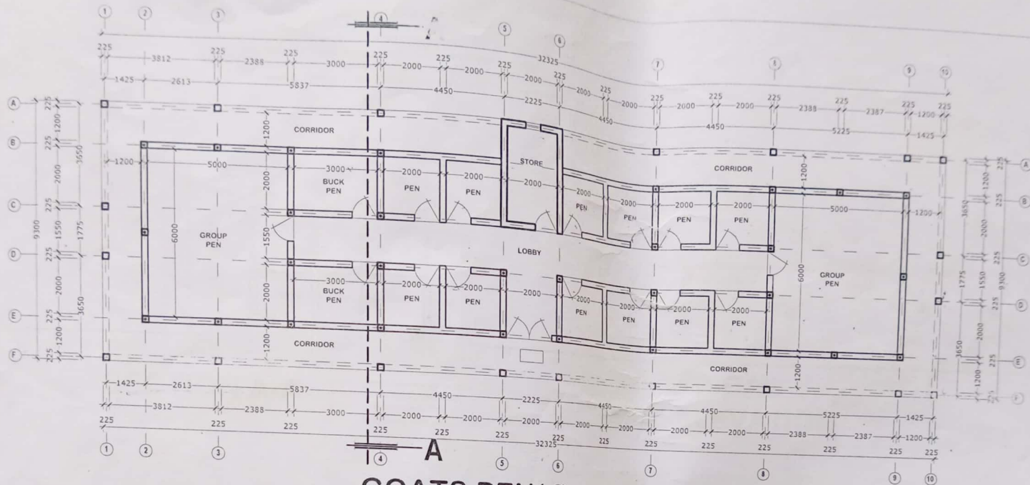
GOATS PEN( floor plan )
