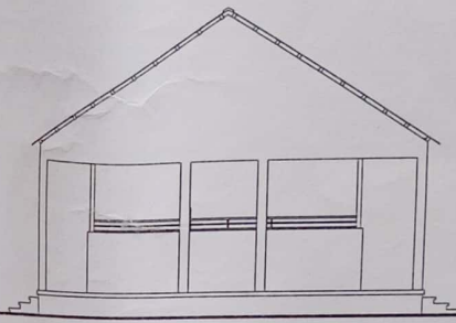
TYPICAL SIDE ELEVATION
