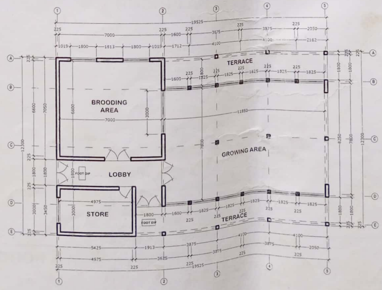
LAYERS PEN ( floor plan )
