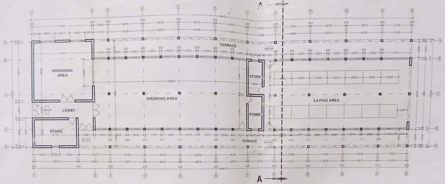
LAYERS PEN ( floor plan )
